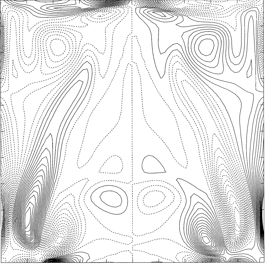
FIG. 10. Contour plot of \omega_1 at the center plane \{x = \frac{1}{2}\} computed using Method B and (4.1). Parameters: \text{Re} = 3200 , t = 15 , CFL = \Delta t/\Delta x = 2.5 , \Delta x = \frac{1}{64} .
