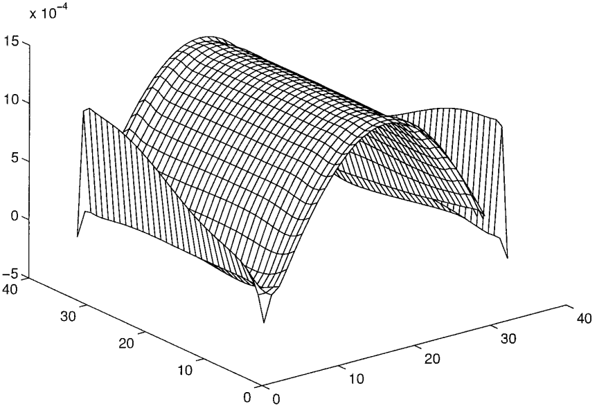
FIG. 4. Numerical error in \omega_2 at the center plane \{x = \frac{1}{2}\} computed using Method B for the full nonlinear problem, using (3.4). Parameters: Re = 100 , t = 5 , \Delta x = \frac{1}{32} .
