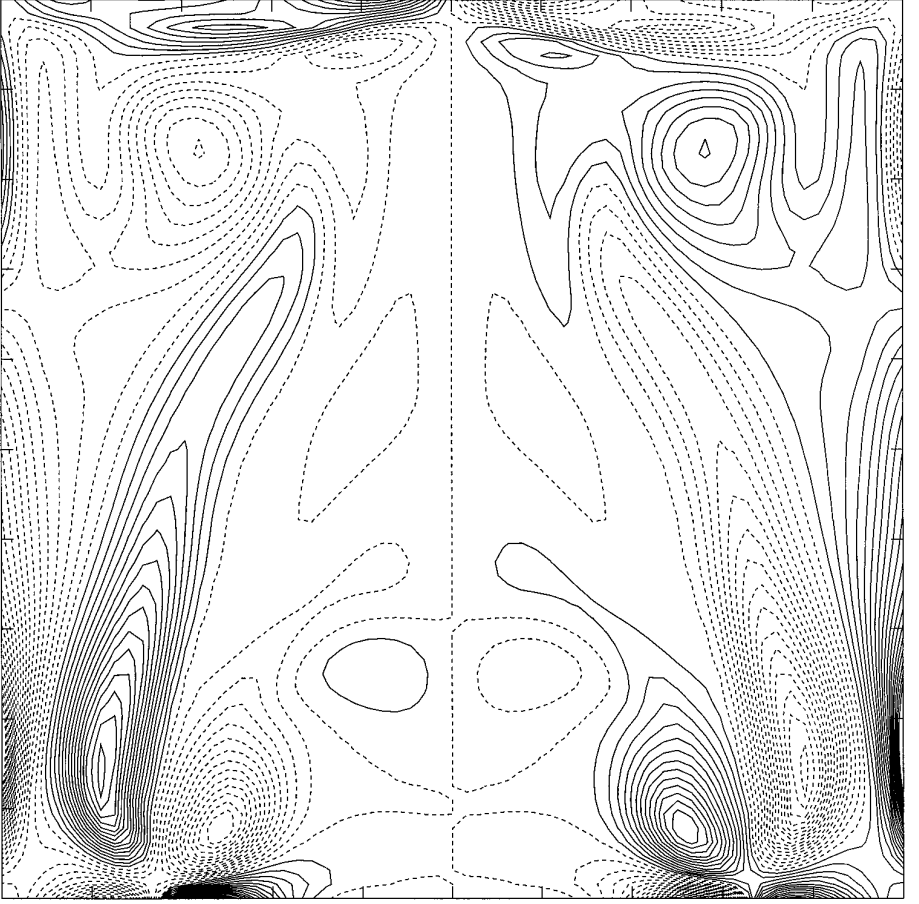
FIG. 13. Contour plot of \omega_1 at the center plane \{x = \frac{1}{2}\} computed using Method A and (4.1). Parameters: \text{Re} = 3200 , t = 15 , CFL = \Delta t/\Delta x = 2.5 , \Delta x = \frac{1}{64} .
