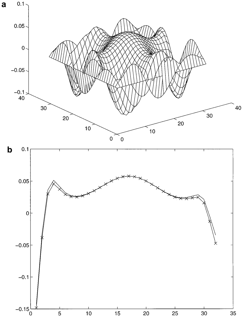
FIG. 2. (a) Numerical error in \psi in 2D for the full Navier–Stokes equation using a similar method and Thom’s formula. Parameters: \text{Re} = 100 , t = 5 , \Delta x = \frac{1}{32} . (b) A cut of the quantity plotted in Fig. 2a at \{x = \frac{15}{32}\} , and comparison with the result when Thom’s formula is replaced by Orszag–Israeli’s formula.
